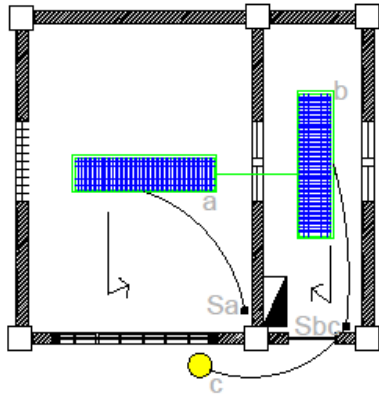
1 LIGHTING OUTLET PLAN E 1 DRAWN NOT TO SCALE
