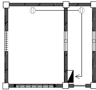
1 CONVENIENCE OUTLET PLAN E 2 DRAWN NOT TO SCALE
