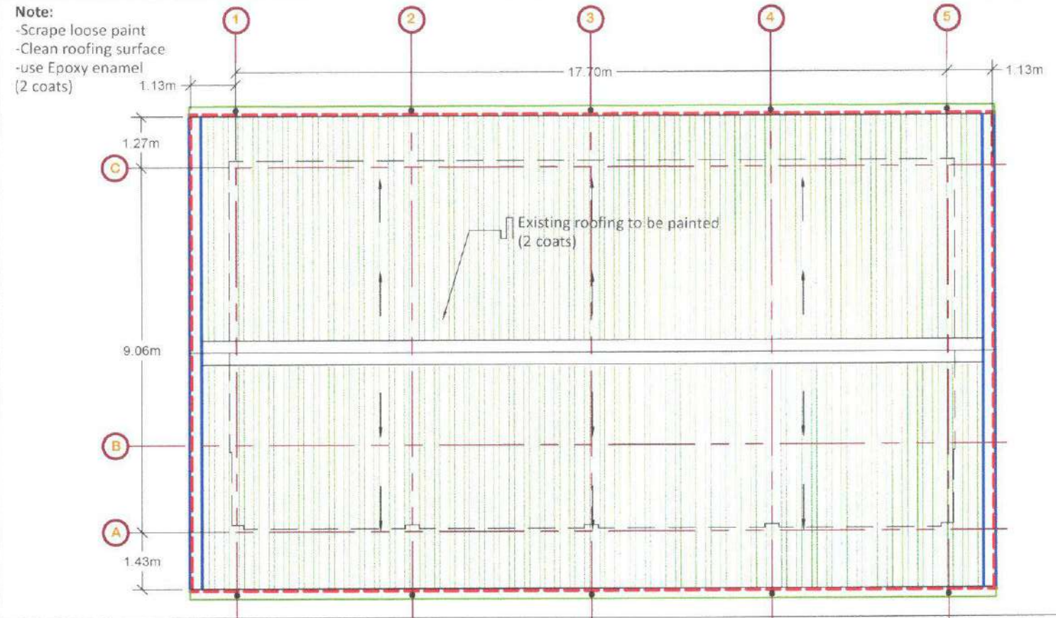
ROOF PLAN SCALE 1 : 1 3 3
