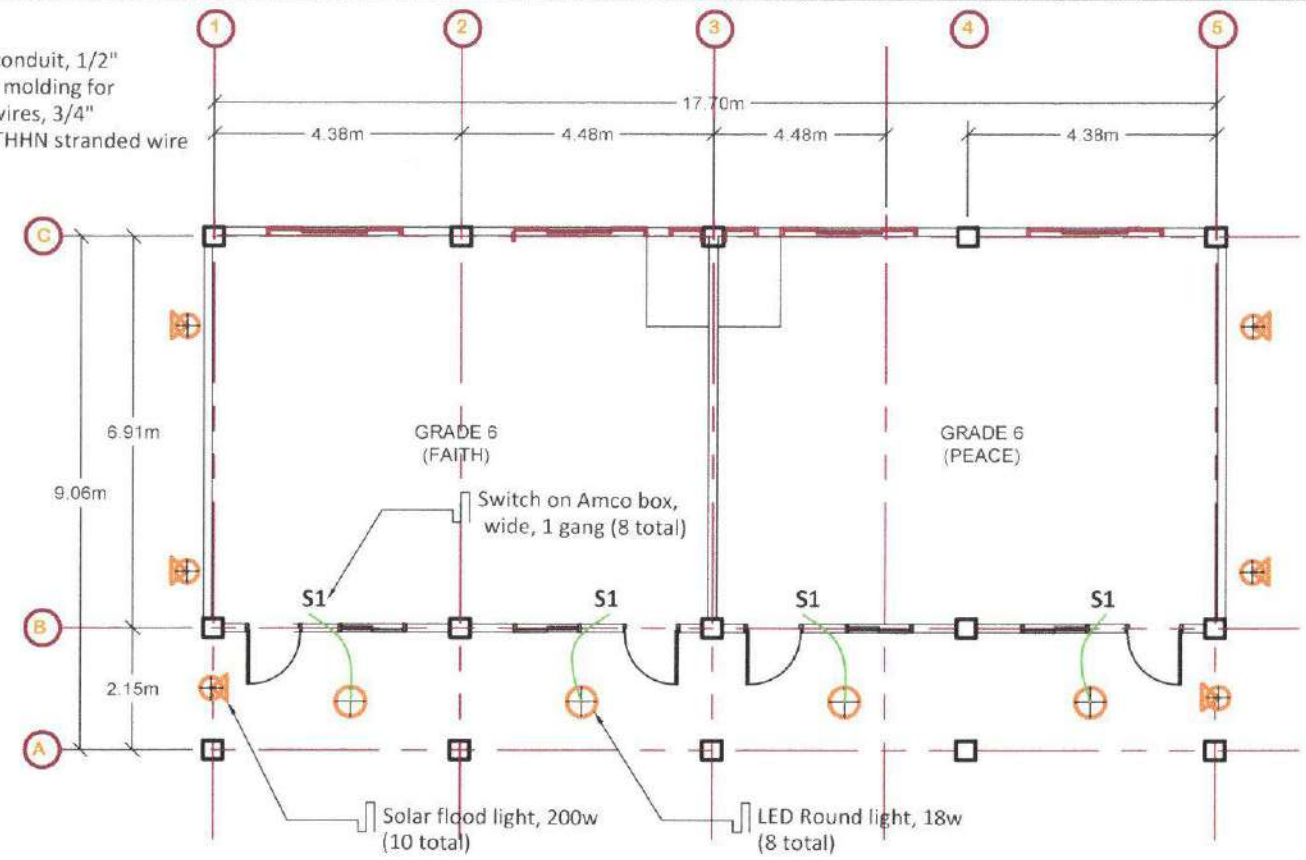
FIRST FLOOR ADDITIONAL LIGHTING LAYOUT SCALE 1 : 1 3 3
