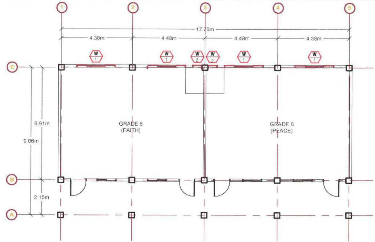
FIRST FLOOR PLAN SCALE 1:133
