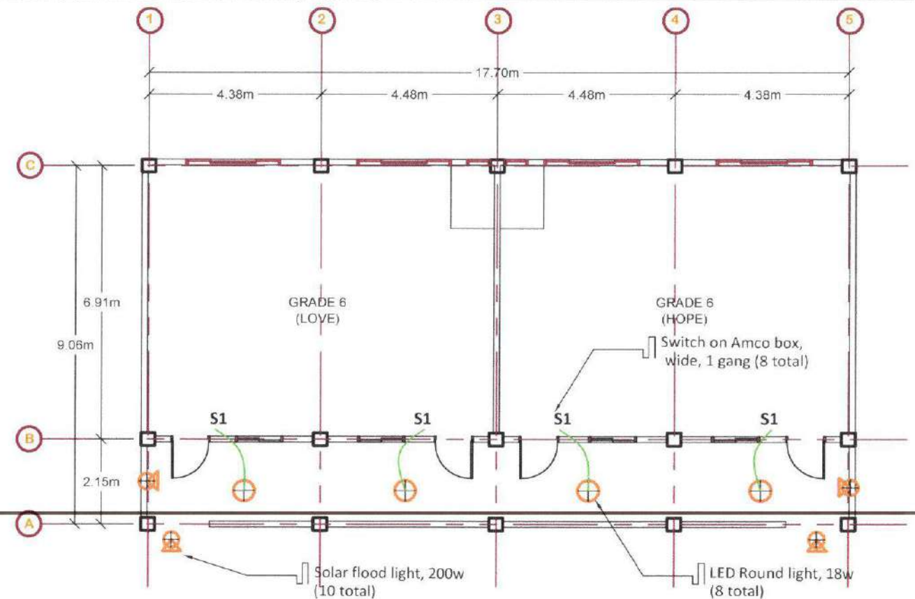
SECOND FLOOR ADDITIONAL LIGHTING LAYOUT SCALE 1 : 1 3 3
