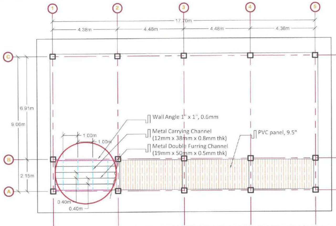
SECOND FLR CEILING AT HALLWAY PLAN SCALE 1 : 1 3 3
