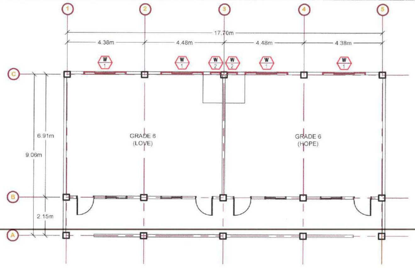
SECOND FLOOR PLAN SCALE 1:133
