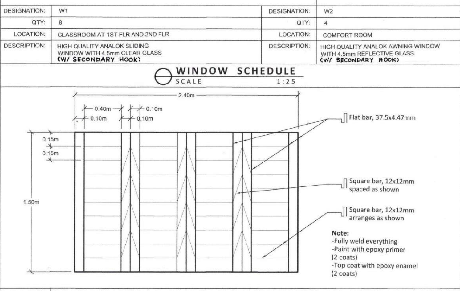
WINDOW GRILL DETAIL SCALE 1:25
