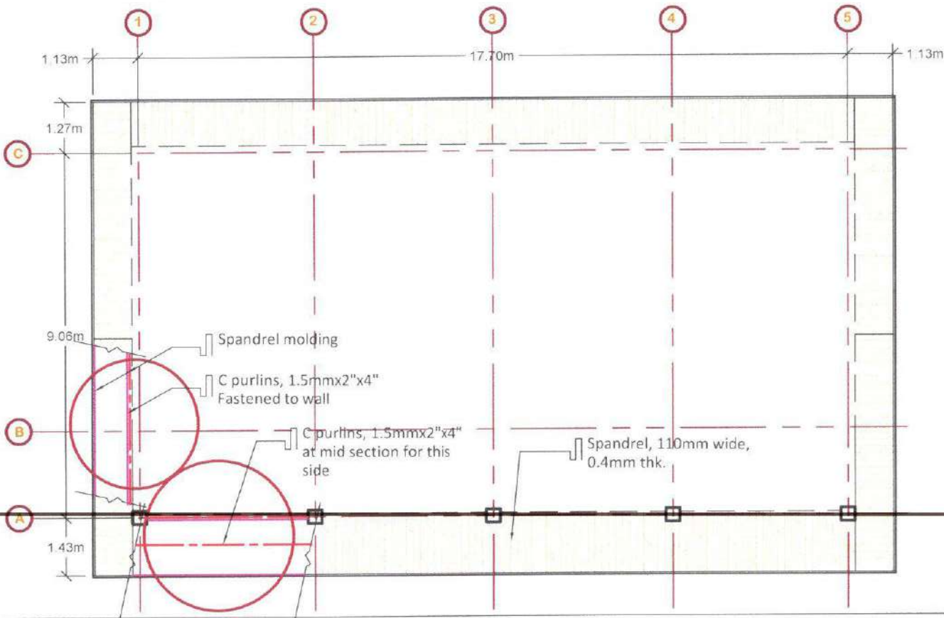
SECOND FLR EAVES/ SOFFIT PLAN SCALE 1 : 1 3 3
