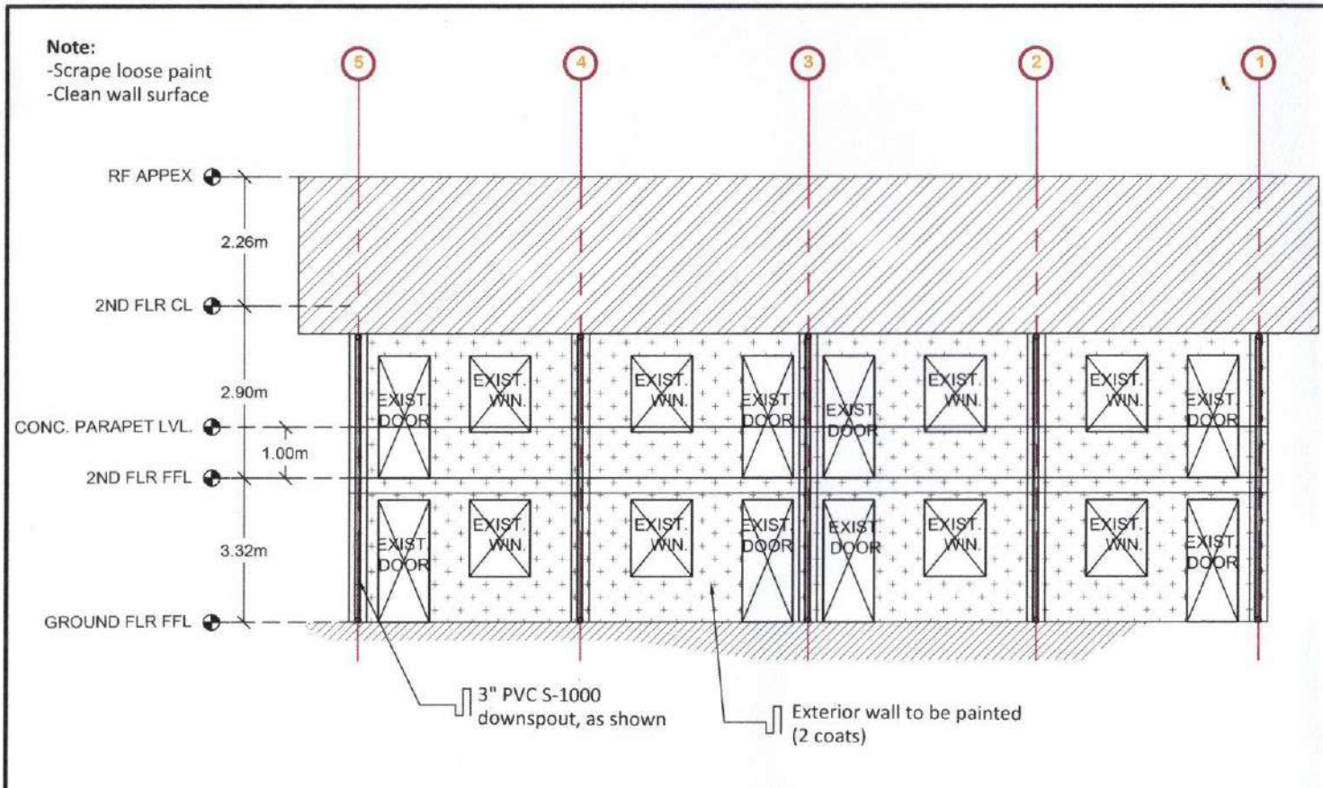
FRONT ELEVATION SCALE 1:133
