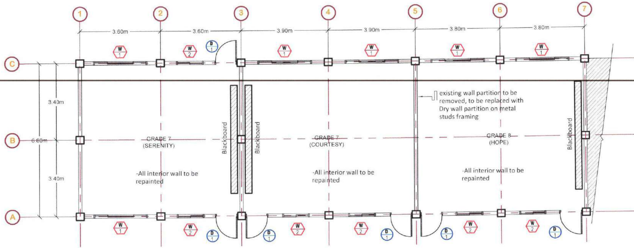
FIRST FLOOR PLAN SCALE 1:100
