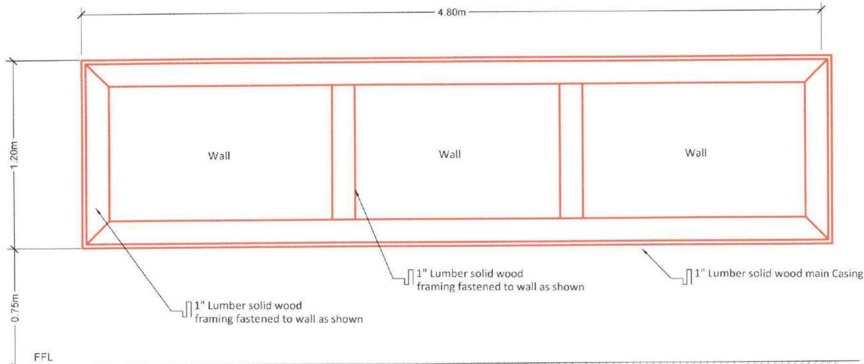
⊙ BLACKBOARD FRAMING ELEVATION SCALE 1:25
