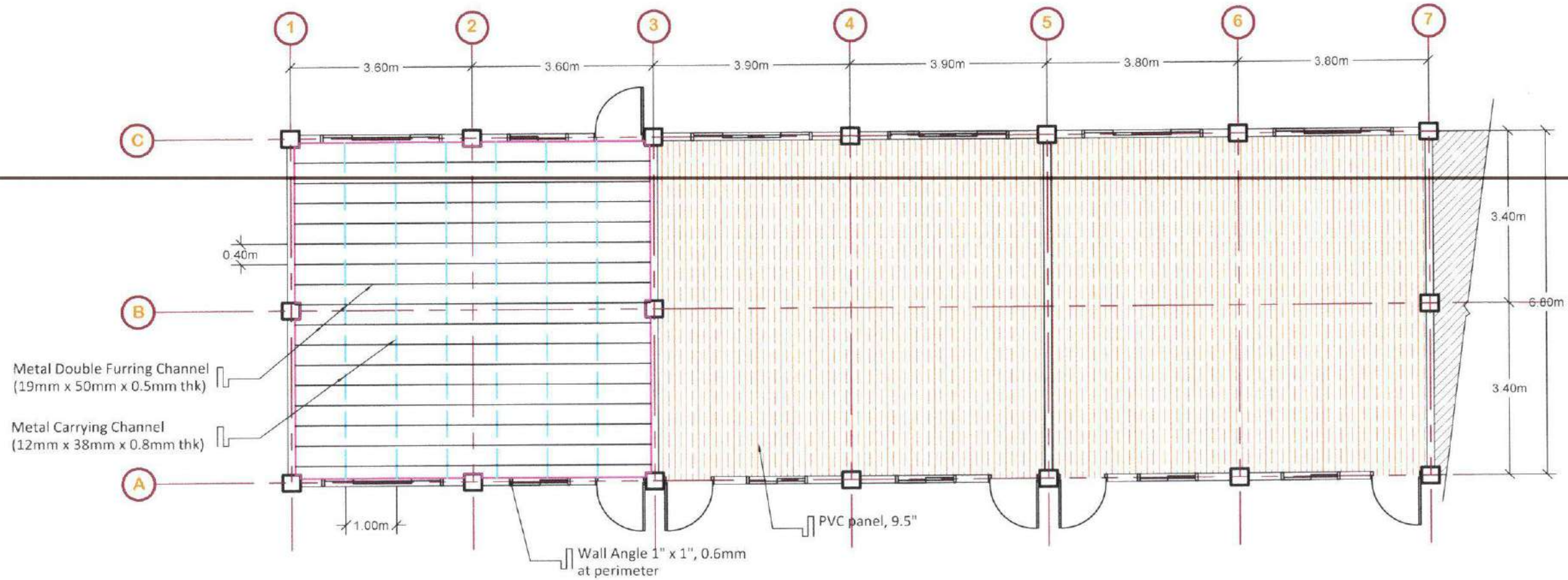
FIRST FLOOR CEILING PLAN SCALE 1 : 100
