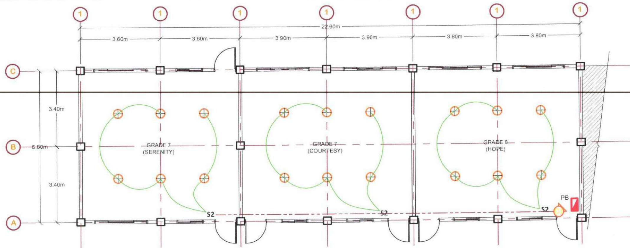
LIGHTING LAYOUT SCALE 1:100
