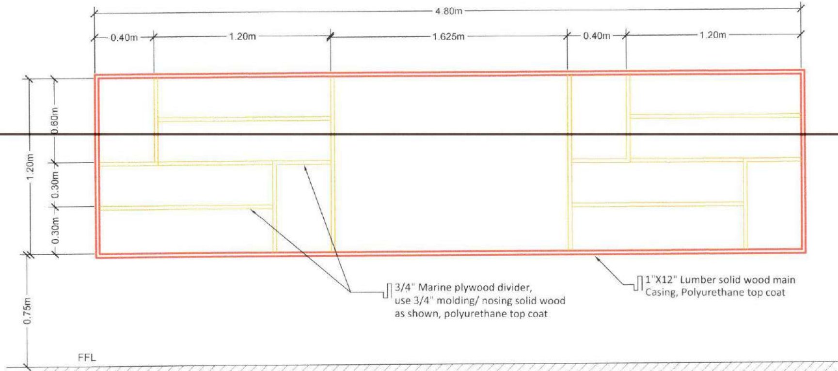
⊙ BLACKBOARD BUILT IN CABINET ELEVATION SCALE 1:25
