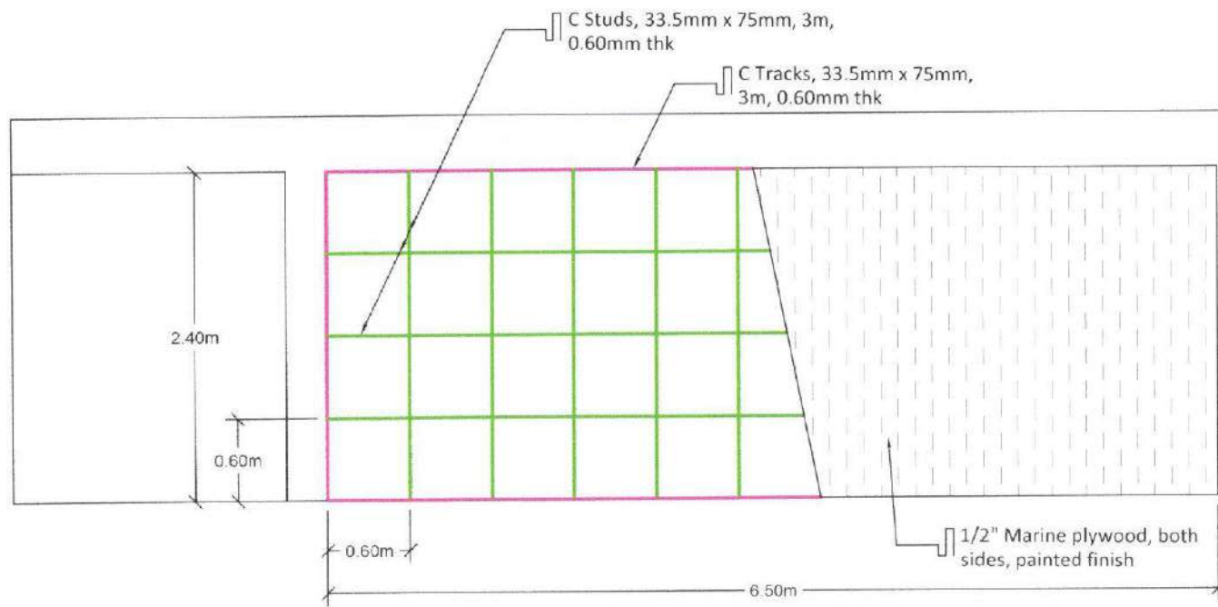
DRY WALL PARTITION DETAIL SCALE 1 : 50
