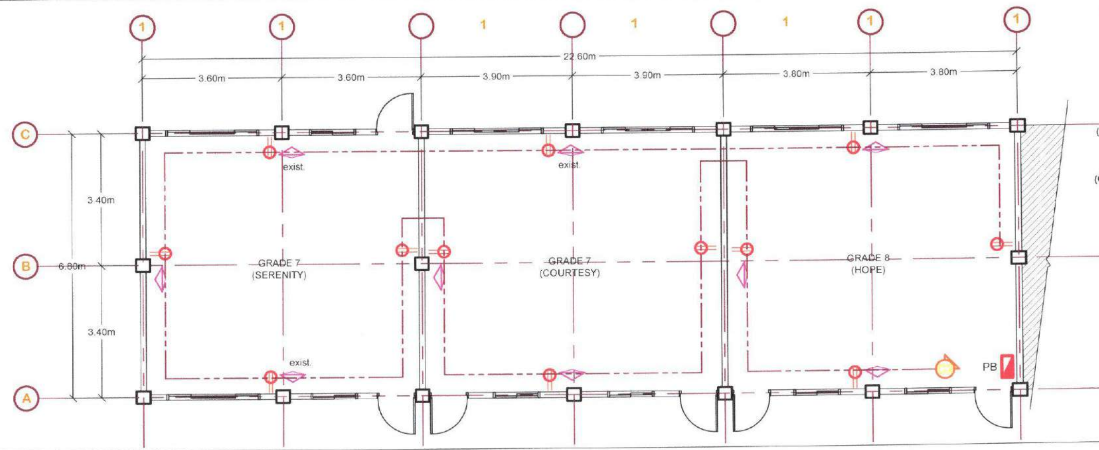
POWER LAYOUT SCALE 1:100
