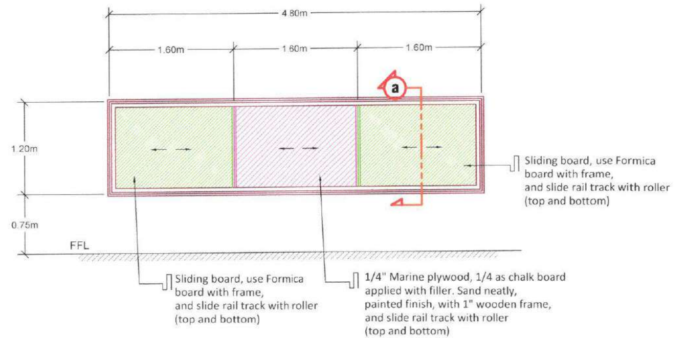
BLACK BOARD ELEVATION SCALE 1 : 50
