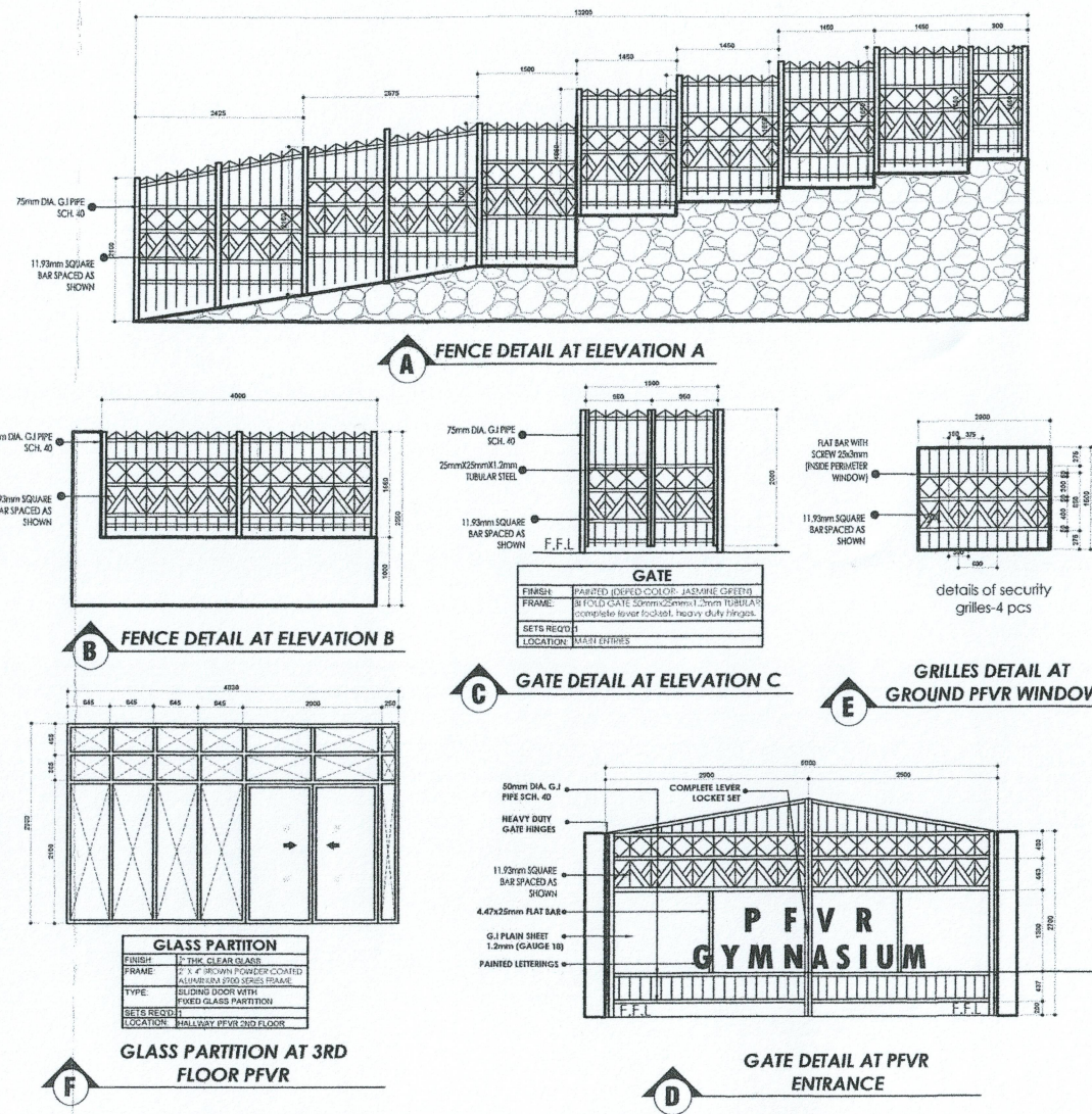
2 BLOW-UP DETAILS SCALE 1:100MTS
