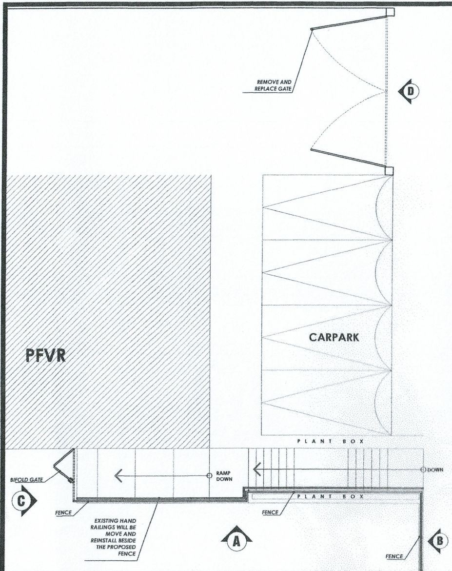
1 GROUND FLOOR PLAN SCALE 1:100MTS
