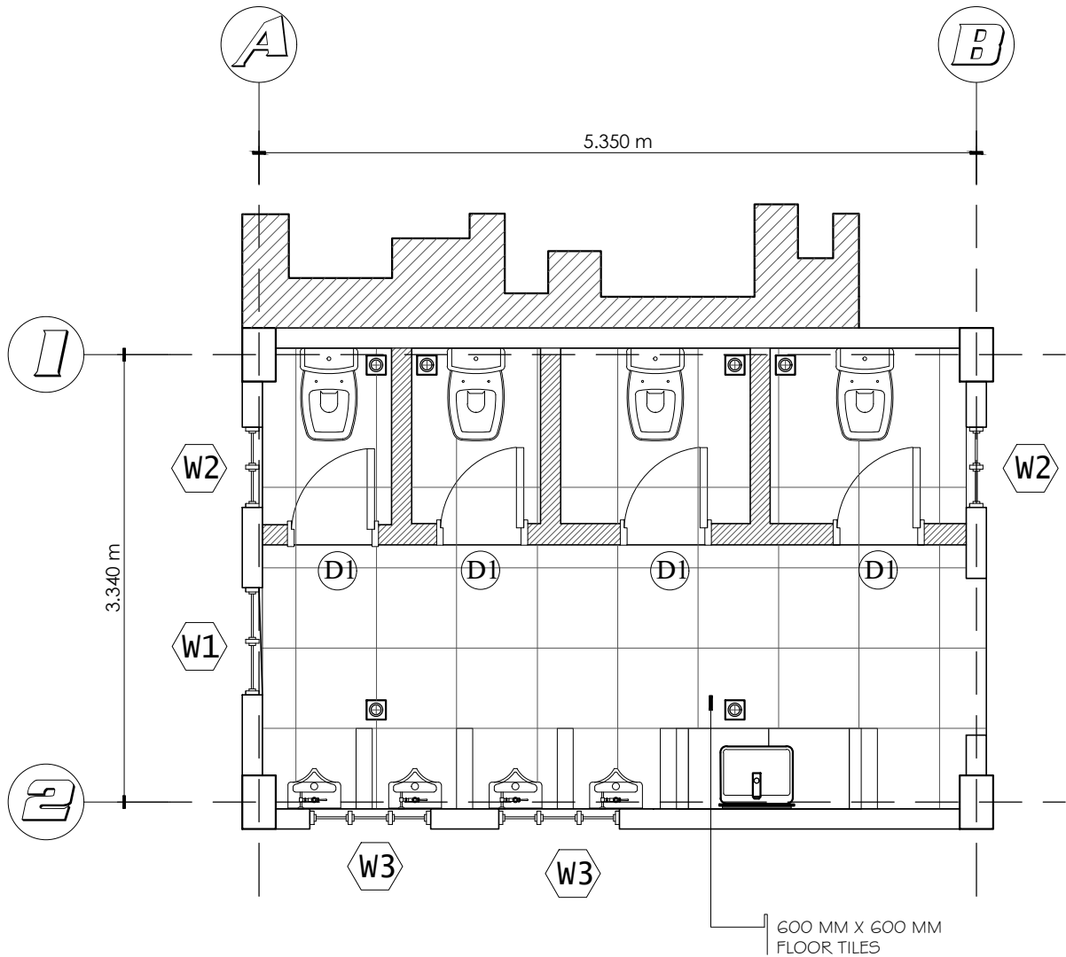
1 COMFORT ROOMS FLOOR PLAN 1 1 SCALE 1:50
