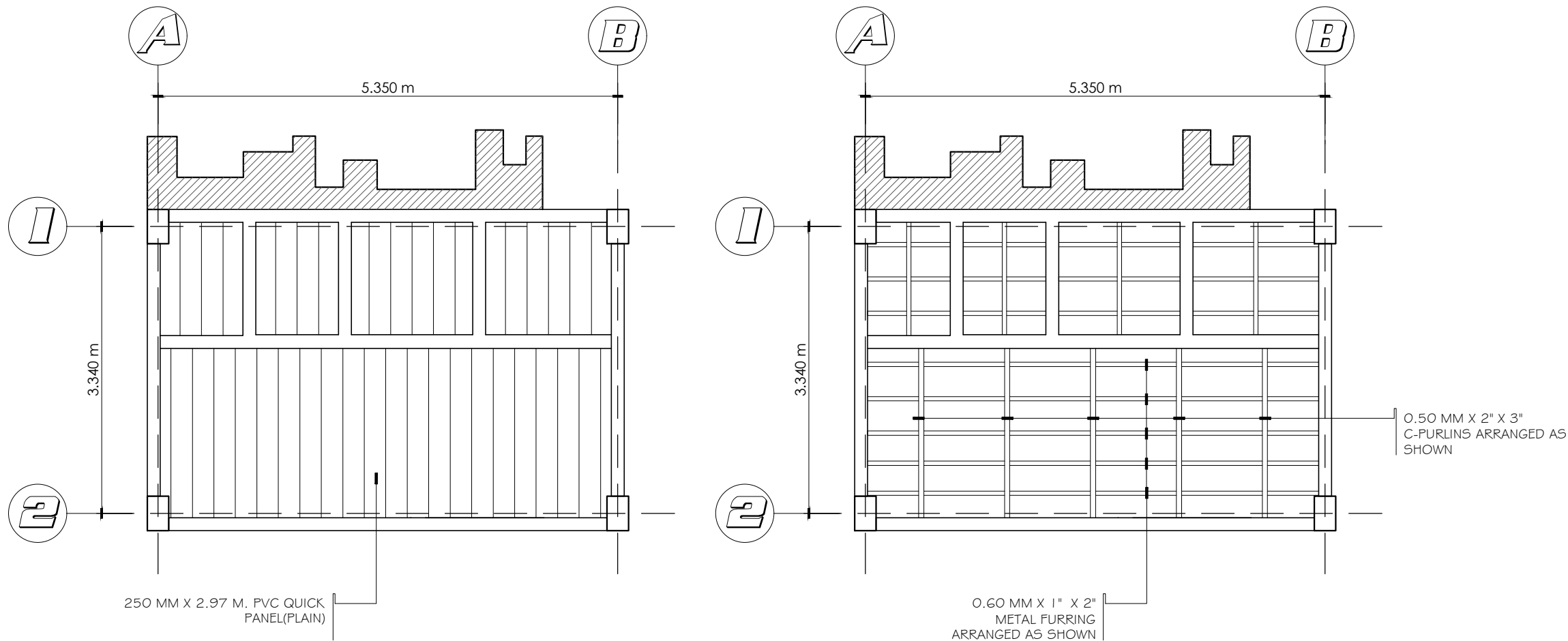
1 COMFORT ROOMS CEILING DETAIL 2 2 SCALE 1:60
